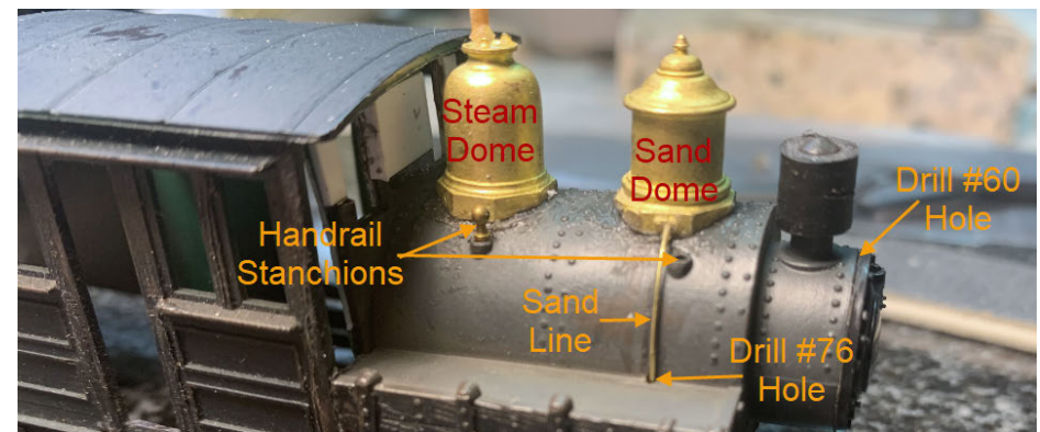
13. I installed a brass sand line. The back stanchions are already in place.
