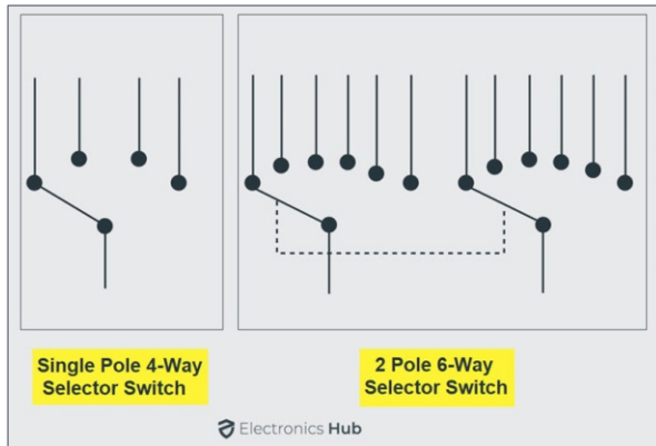
7. Circuit diagrams for rotary selector switches.
