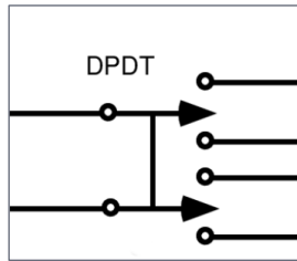
3. Circuit diagram for double-pole double-throw switch with an off position.
