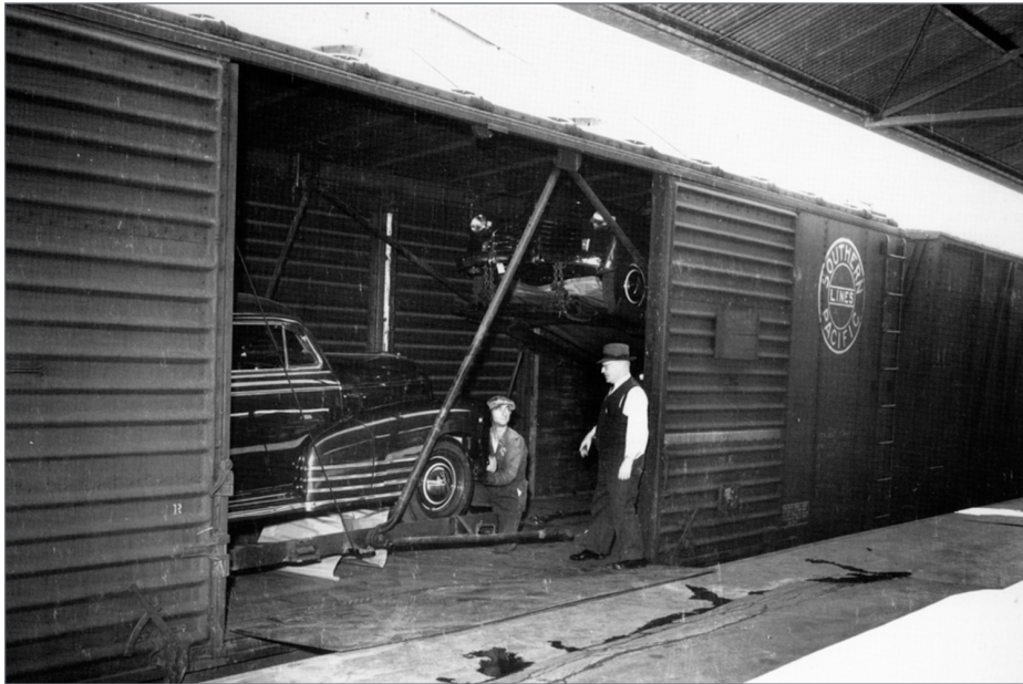
7. An important part of automobile industry traffic was and is assembled or set-up vehicles, shipped to all parts of the country. These cars are being loaded into a boxcar with auto racks at Chevrolet's Melrose Assembly plant in Oakland, California. SP photo
