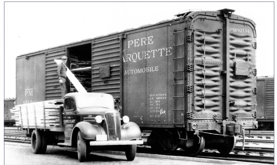
19. This photo shows an employee of Schweikart Lumber unloading lumber from a 40-foot automobile car at Ashland, Kentucky, about 1940. You can see inside that a great deal of lumber remains. C&O Historical Society
