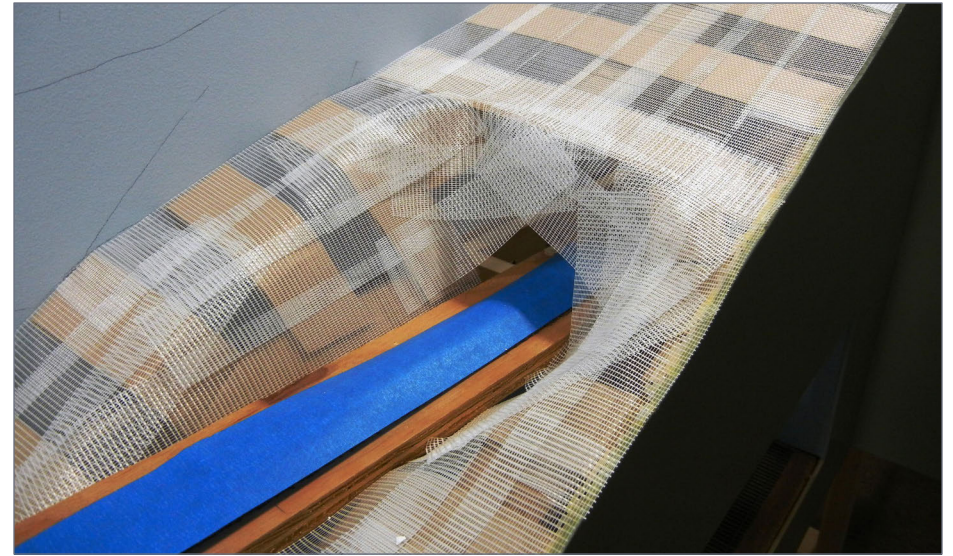
7. Here's a hillside covered with FibaTape. I constructed the cardboard scenic supports using the same technique of building up the hill, then working-in the cuts, abutments, and tunnel portals later.
