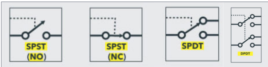
2. Circuit diagrams, left to right: Single-pole single-throw, normally open; single-pole single-throw, normally closed; single-pole, double-throw; double-pole, double-throw.
