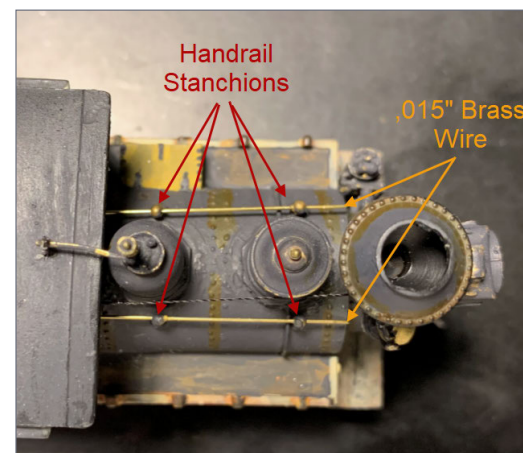
14. The handrails are installed.
