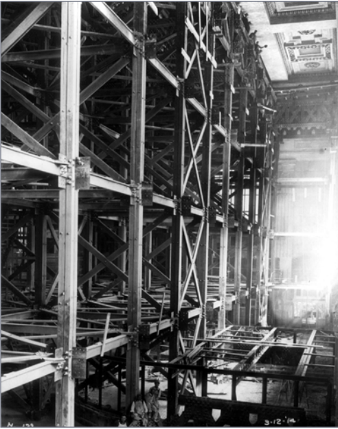
14. Scaffolding ready to be removed from inside the completed Grand Lobby.
