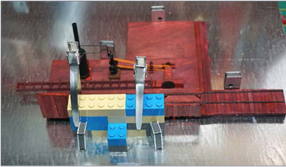
29. Lego blocks and magnets hold parts square.
