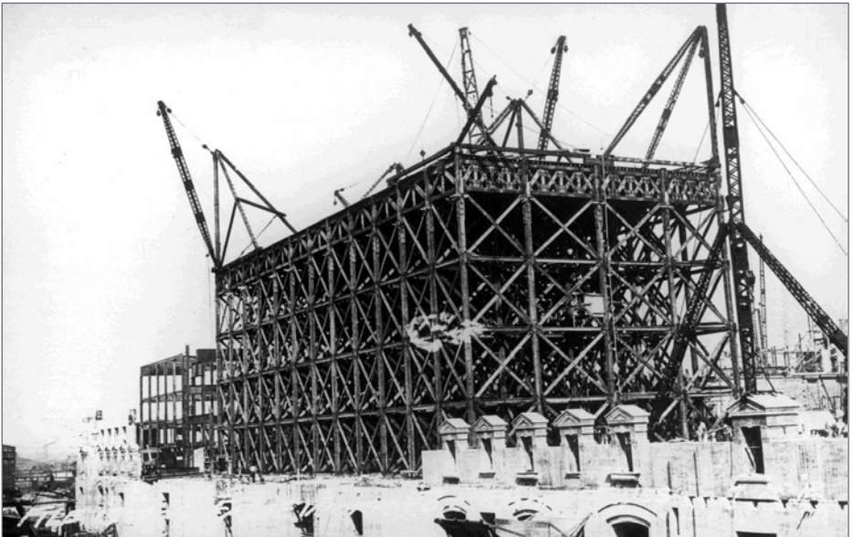
13. Scaffolding used to construct the Grand Lobby.
