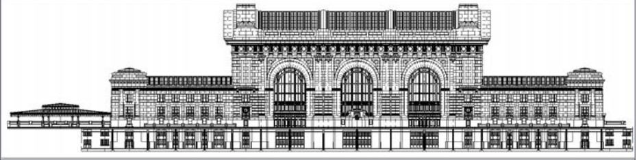
23. The final CAD drawing of the South Elevation
